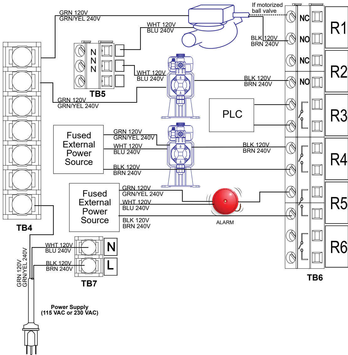
Figure 15 W610 AC Power & Relay Output Wiring
